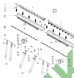
ETB-011590, Rama nośna (2/2)
