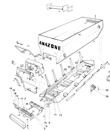
ETB-011547, Wylot
