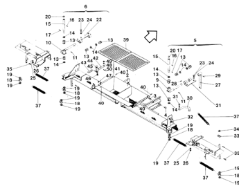
ETB-011589, Rama nośna (1/2)
